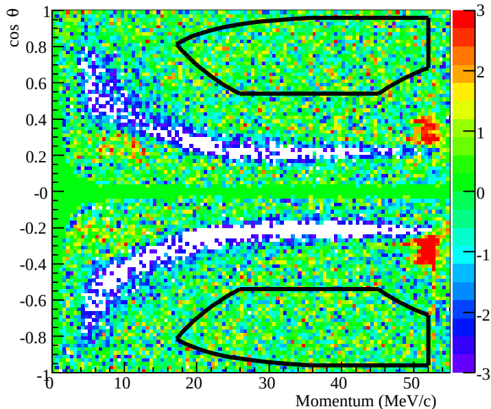
Normalized Fit Residuals (data - MC)/ \sigma
