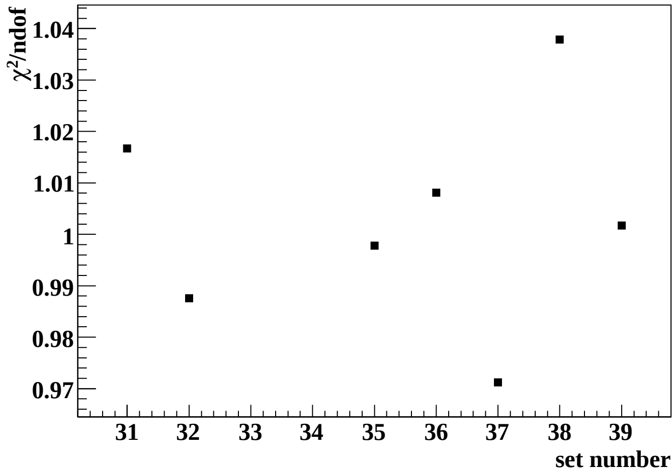
\chi^2/\text{ndof} for Michel spectrum fits
