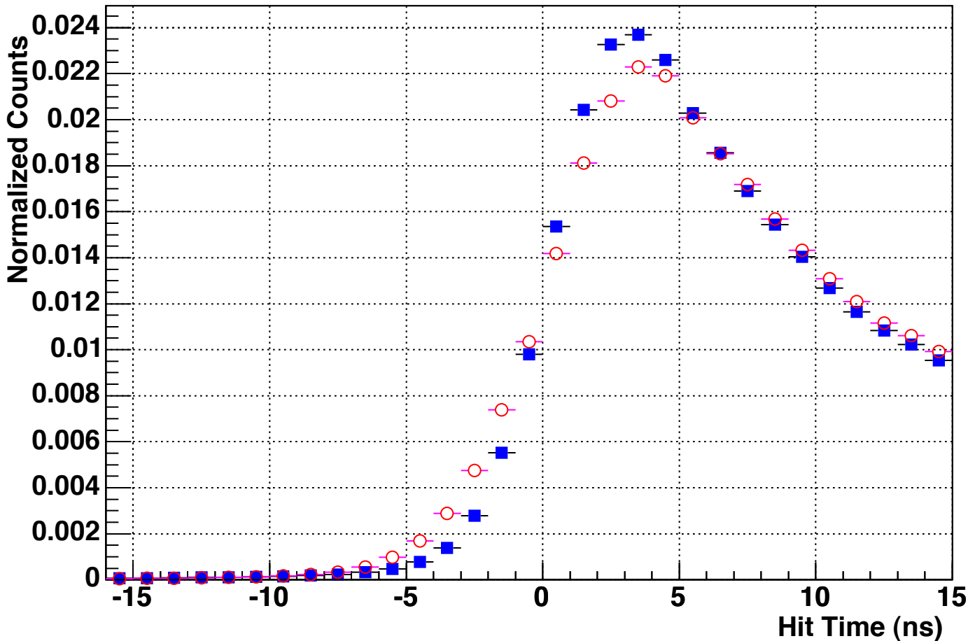
TDC Hit Time: Data (blue) MC (red)
