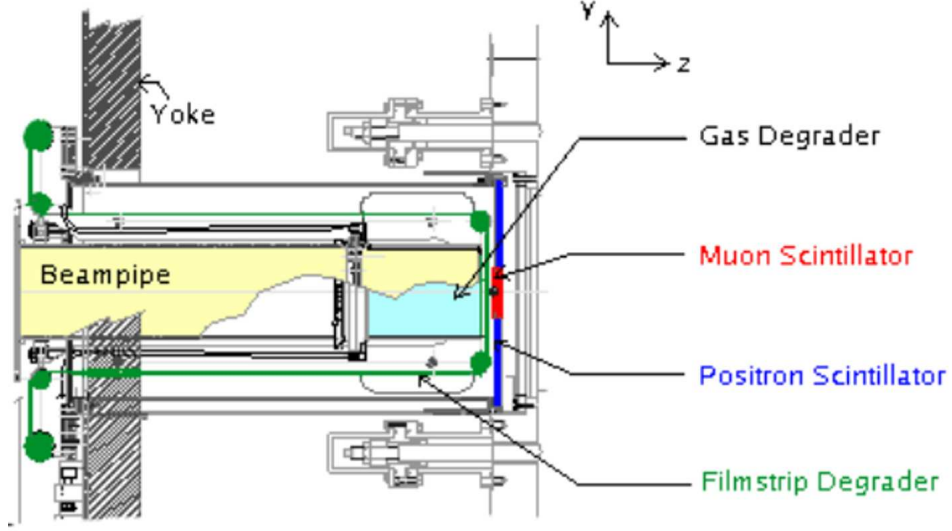
Figure 2.12: Beam package for the upstream end of the detector[57]. The beam did not encounter material until the upstream window of the gas degrader ( z = -103.2 cm). At this location the magnetic field strength was 1.5 T.
