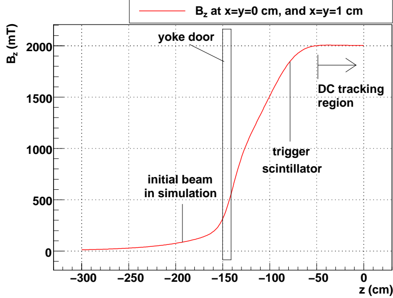
Figure 6.2: Longitudinal ( B_z ) components from the field map used for the analysis. These are produced from an Opera finite element analysis[87].
