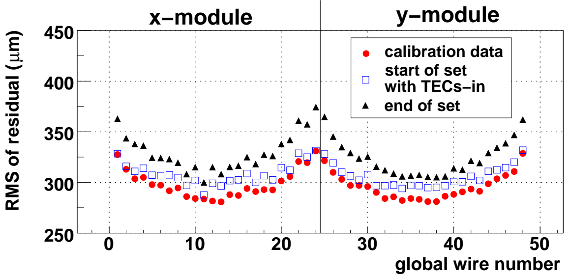
Figure G.6: Resolution (RMS of residual distribution, when wire is excluded from fit). The calibration data corresponds to newly built sense planes. The beginning and end of the set with TECs-in corresponds to a time period of one week, over which the planes aged significantly.
