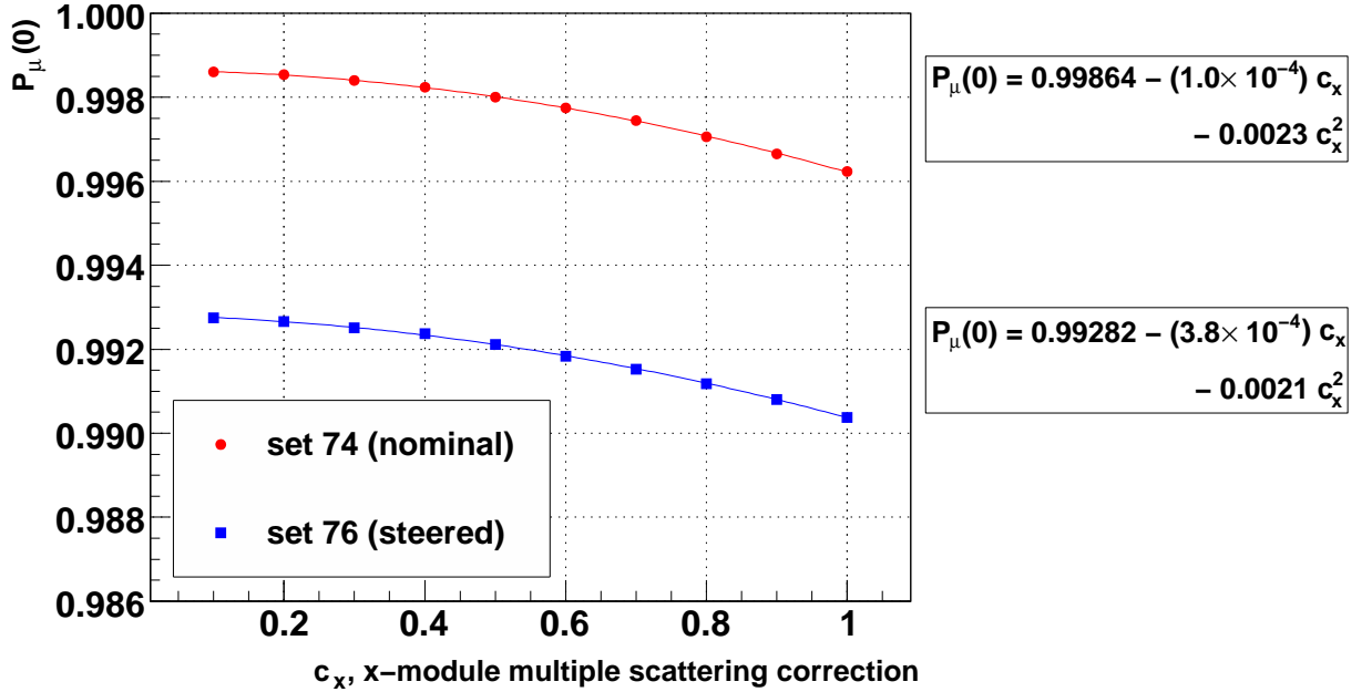
Figure 6.8: Sensitivity of the simulation's P_\mu(0) to c_x , the multiple scattering correction factor in the x -module. The ratio c_x/c_y = 0.64/0.48 was maintained.
