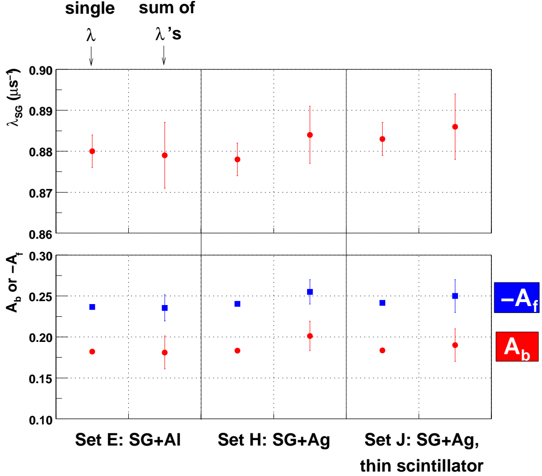
Figure H.3: Effect on \lambda_{SG} , A_b and A_f when a second exponential scintillator depolarisation with \lambda_{scint} = 0.0132\mu\text{s} is included.
